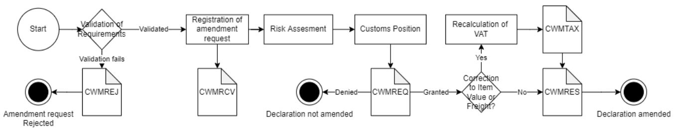
Figure 1 – Amendment flow
